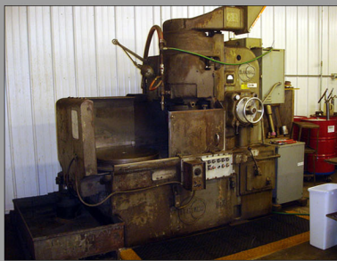
30" Blanchard No. 18 Rotary Surface Grinder. Serial No. 10895.
