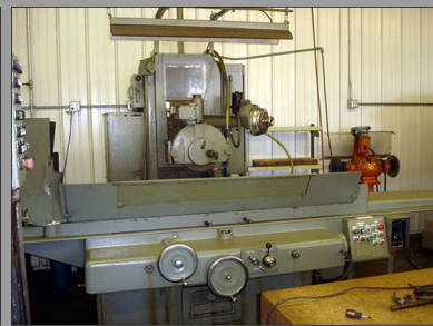
16" x 48" Gallmeyer & Livingston Model 670 Hydraulic Surface Grinder. Serial No. 670120, Incremental downfeed.
