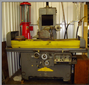
22" x 24" Elb Model SWB6VAI Hydraulic Surface Grinder
